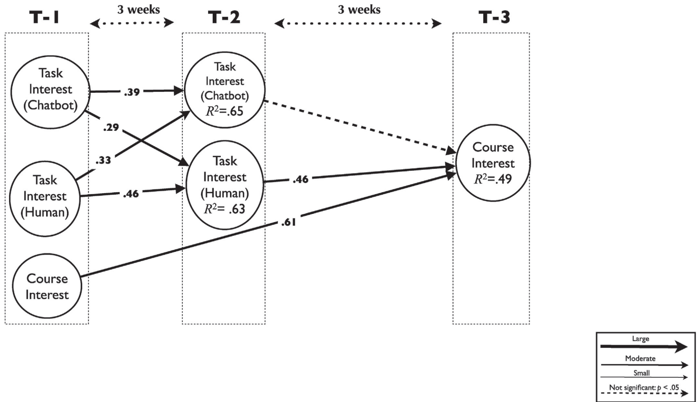
Fig. 2. Significant predictive coefficients between task interest under Chatbot and Human partner conditions as they predict to T3 course interest. Note: All coefficients are \beta s; The dashed arrow represents the tested path that was not significant ( p < 0.05 ).
